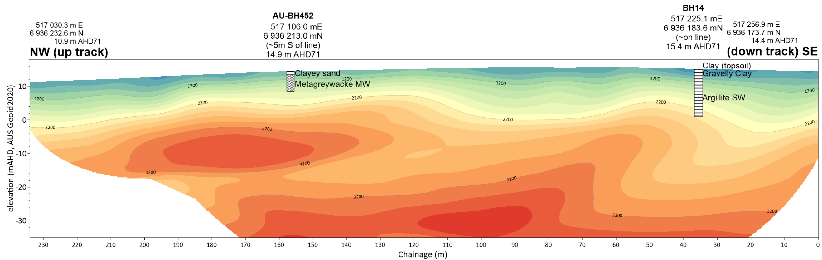
Seismic Refraction data limits
